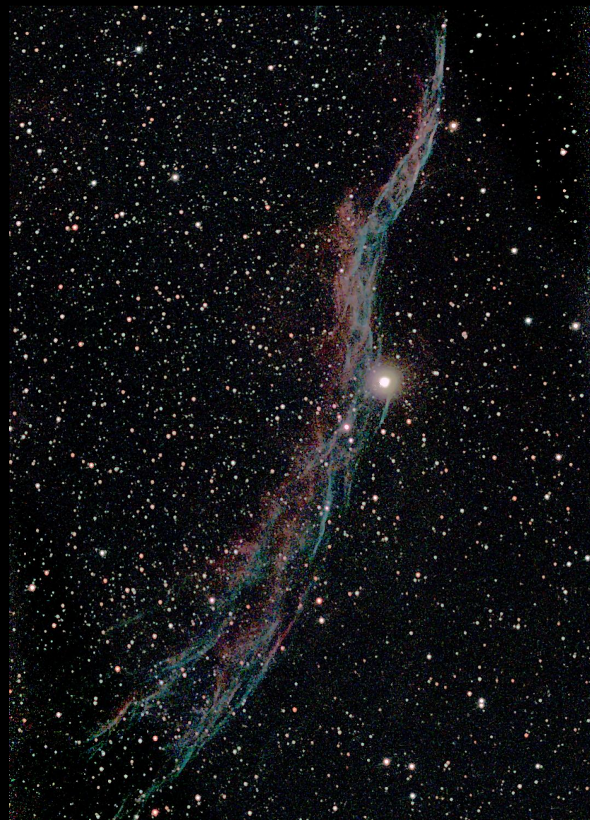
NGC 6960, Western Veil, in Cygnus, 17-Oct-2024, 61 min
